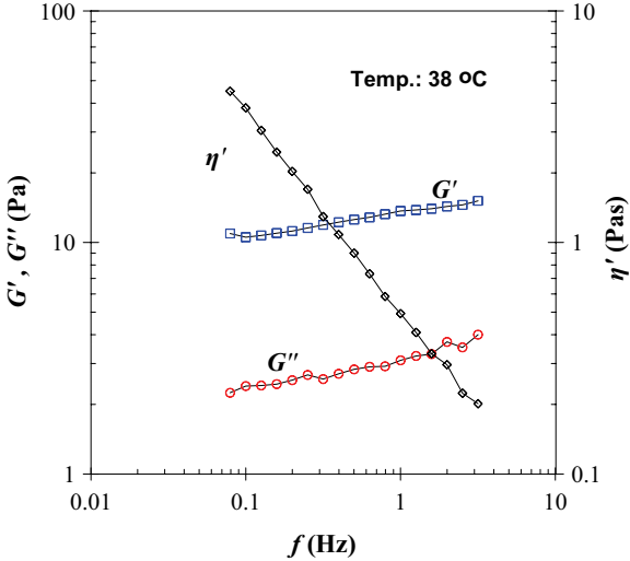
Figure 4. Viscoelastic behaviour of the normal SF for strain value 0.01 ( \gamma\% = 1\% ).
