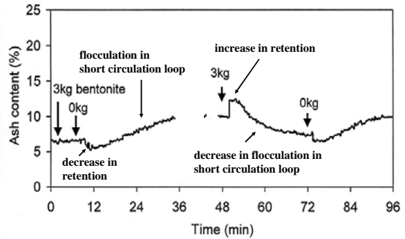
Fig.6. Retention of calcium carbonate fillers, expressed as ash content, on a Fourdrinier pilot machine 17 . CPAM = 0.5 mg/g. Reducing bentonite dosage to zero reduces filler retention initially (as expected), but this decrease is followed by an increase on the time scale of whitewater recirculation, implying flocculation of fillers, followed by entrapment in the sheet on subsequent pass through the machine. This behavior is reversible and reproducible as shown by subsequent step changes in bentonite dosage.
