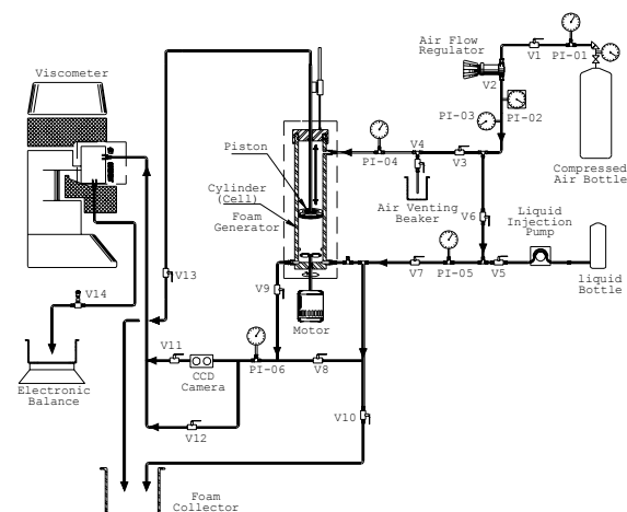
Fig. 2 Schematics of the Foam Generator/ Viscometer
