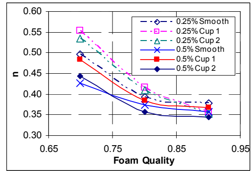
Fig. 13 Flow behavior index versus foam quality, polymer concentrations and cup-rotor assemblies
