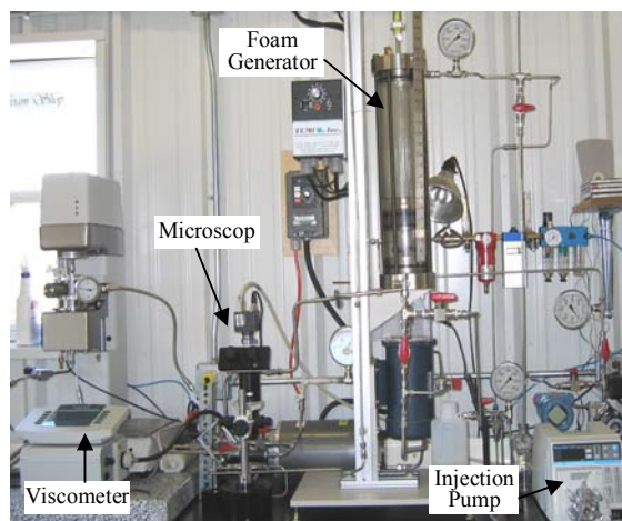
Fig. 1 Foam Generator/ Viscometer
