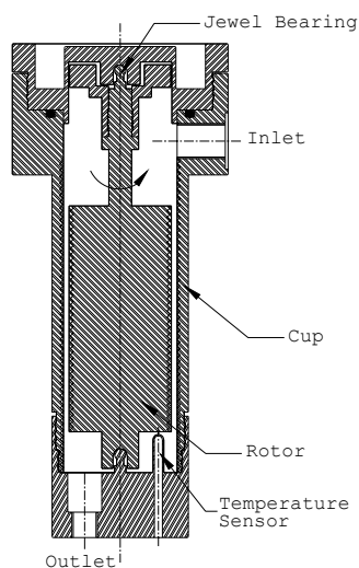
Fig. 3 Rotor-cup assembly of RS-300
