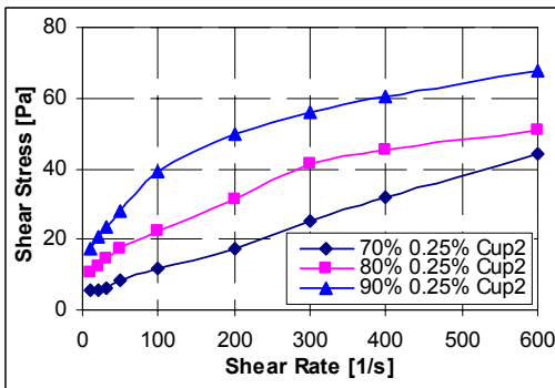
Fig. 10 Polymer foam (0.25%) rheology measured using more roughened cup-rotor assembly #2
