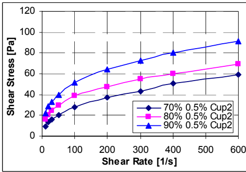
Fig. 11 Polymer foam (0.5%) rheology measured using more roughened cup-rotor assembly #2
