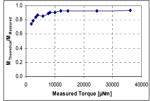
Fig. 4 Viscometer calibration curve obtained at \gamma=400 \text{ s}^{-1}
