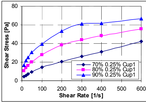
Fig. 8 Polymer foam (0.25%) rheology measured using less roughened cup-rotor assembly # 1
