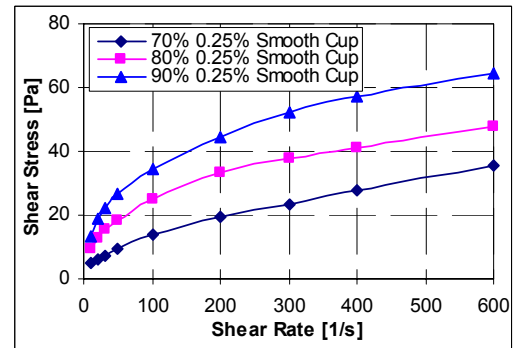
Fig. 6 Polymer foam (0.25%) rheology measured using smooth cup-rotor assembly
