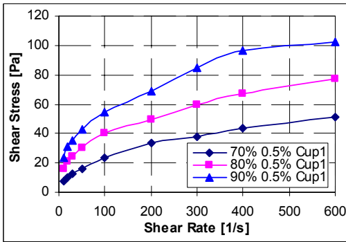
Fig. 9 Polymer foam (0.5%) rheology measured using less roughened cup-rotor assembly # 1
