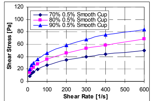
Fig. 7 Polymer foam (0.5%) rheology measured using smooth cup-rotor assembly
