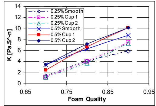
Fig. 12 Flow consistency index versus foam quality, polymer concentrations and cup-rotor assemblies
