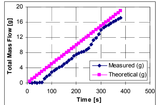
Fig. 5 Total mass flow through the viscometer versus time for an 80% quality 0.25% polymer foam
