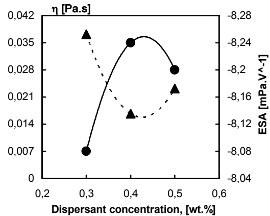
Figure 6. Effect of addition of PMA-NH 4 on the (▲) viscosity and (●) ESA for a 43-vol% alumina suspension at pH 9.
