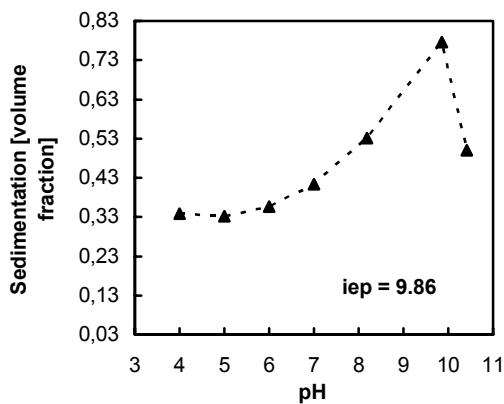
Figure.5. pH dependence of (▲) sedimentation volume for a 2-vol% alumina suspension.
