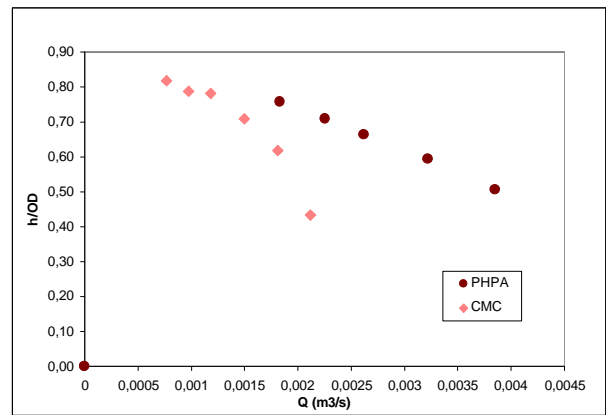
Figure 3- Bed Erosion With Low Viscosity Fluids – Concentric Annulus
