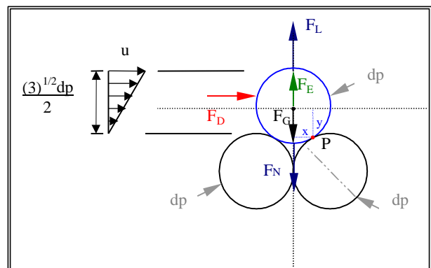
Figure 9 – Schematic showing the forces acting upon a particle in the imminence of moving
