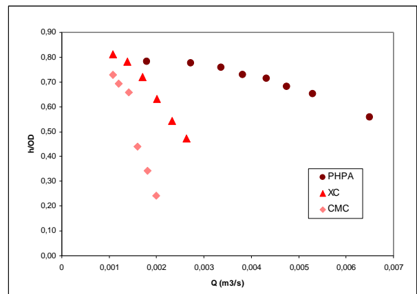
Figure 5- Bed Erosion With High Viscosity Fluids – Concentric Annulus
