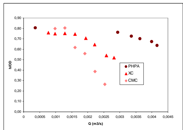
Figure 4- Bed Erosion With Average Viscosity Fluids – Concentric Annulus
