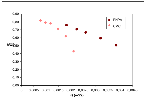
Figure 6- Bed Erosion With Low Viscosity Fluids – Eccentric Annulus
