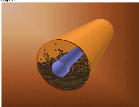
Figure 1 – Cuttings Bed Formation in Horizontal Annulus
