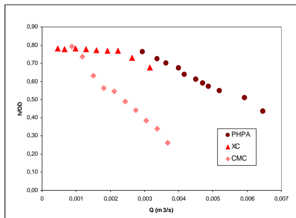
Figure 7 - Bed Erosion With Average Viscosity Fluids – Eccentric Annulus
