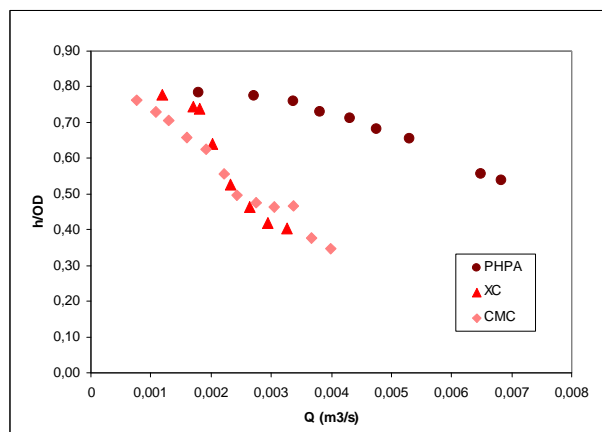
Figure 8 - Bed Erosion With High Viscosity Fluids – Eccentric Annulus
