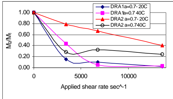
Fig.5 Molecular weight ratio ( M_2/M_1 ) of the sheared to the unsheared polymers.
