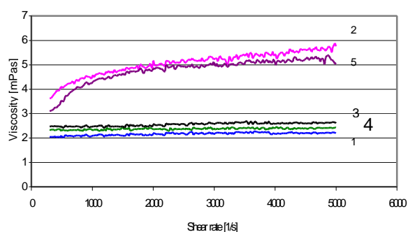
Figure 2 Viscosity of 1000 ppmw DRA1 exposed to different shear rates at 40°C, 1) DO, 2) 0 sec -1 , 3) 6790 sec -1 , 4) 13582 sec -1 and 5) 3395 sec -1
