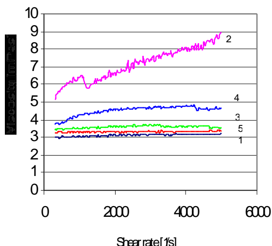
Fig.1 Viscosity of 1000 ppmw DRA1 exposed to different shear rates at 20°C 1) DO, 2) 0 sec -1 , 3) 7690 sec -1 , 4) 3395 sec -1 , 5) 13582 sec -1 .
