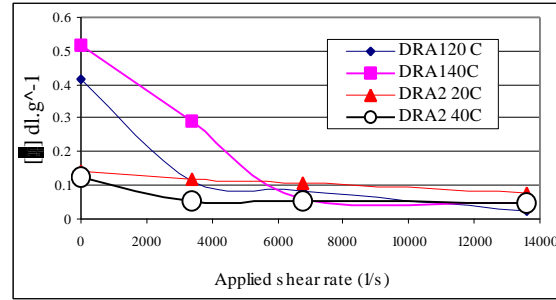
Figure 4 [\eta] for the different sets of the applied shear rates on DRA1 and DRA2 at 20 and 40°C.
