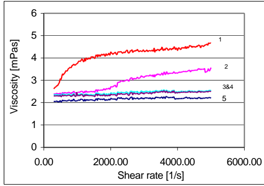
Figure 3 Viscosity of 1000 ppmw DRA2, exposed to different shear rates at 40C 1) 0 sec-1, 2) 3395 sec-1, 3) 6791 sec-1, 4) 13581 sec-1, 5) DO
