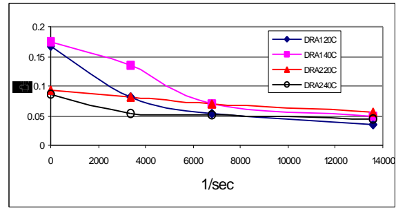
Figure 6 Volume fraction \alpha of the swollen polymer.
