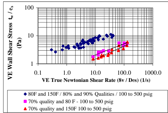
Figure 11. VE Foam Master Flow Curve – Stiffer Foam
