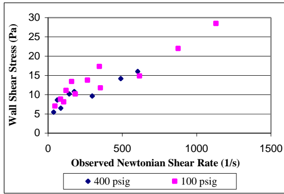
Figure 8. Effect of Pressure on Foam Rheology – 100 °F / 90% quality – Baseline Tests.
