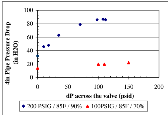
Figure 2. Effect of Foam Generation on Foam Rheology – Stiffer Foam
