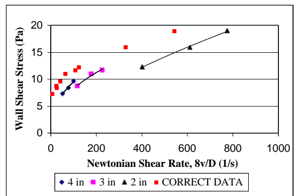
Figure 5 – Slip Correction – 300 psig / 100F / 80% Quality – Baseline Tests
