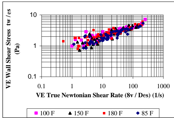
Figure 10. VE Foam Master Flow Curve –60% to 90% Quality – 100 to 650 psig Baseline Tests
