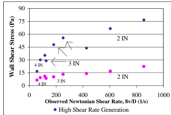
Figure 3. Effect of Foam Generation on Rheology – 90% quality/100 psig/85°F
