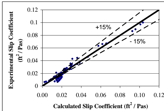
Figure 6. Comparison Between experimental and Calculated Slip Coefficient
