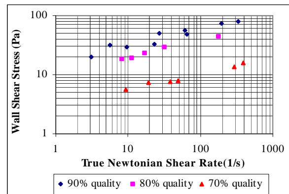
Figure 7. Effect of Quality on Foam Rheology – 300psig / 80°F – Stiffer Foam
