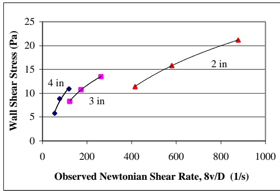
Figure 4. Example of Slippage at Wall in Pipe Flow – 100psig / 150°F / 90% Quality Foam – Baseline Tests
