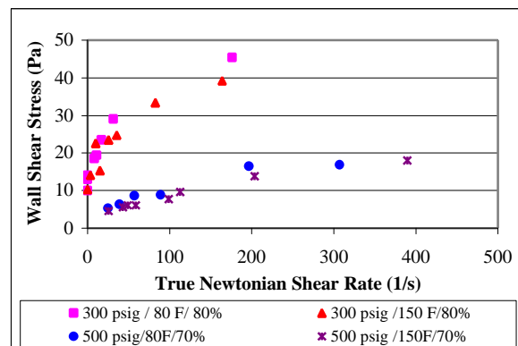
Figure 9. Influence of Temperature on Foam Rheology – Stiffer Foam
