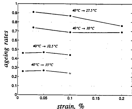
Fig. 1. The influence of strain used in DMA on the ageing rate \mu , for PVAc following indicated on curves thermal histories.
